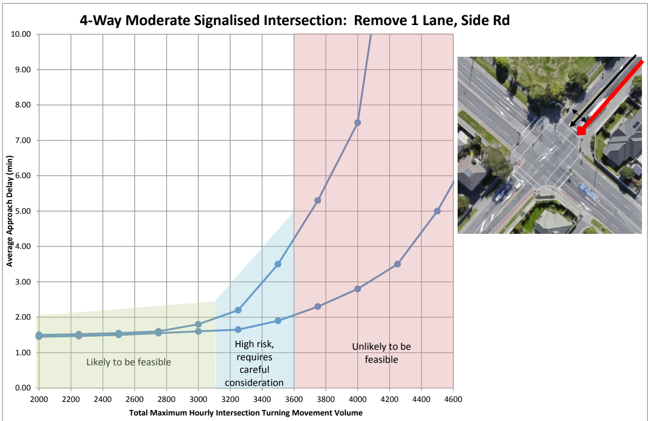
Figure 9: 4-way Moderate Signalised Intersection: Removing Right Turn Lane from Side Road
