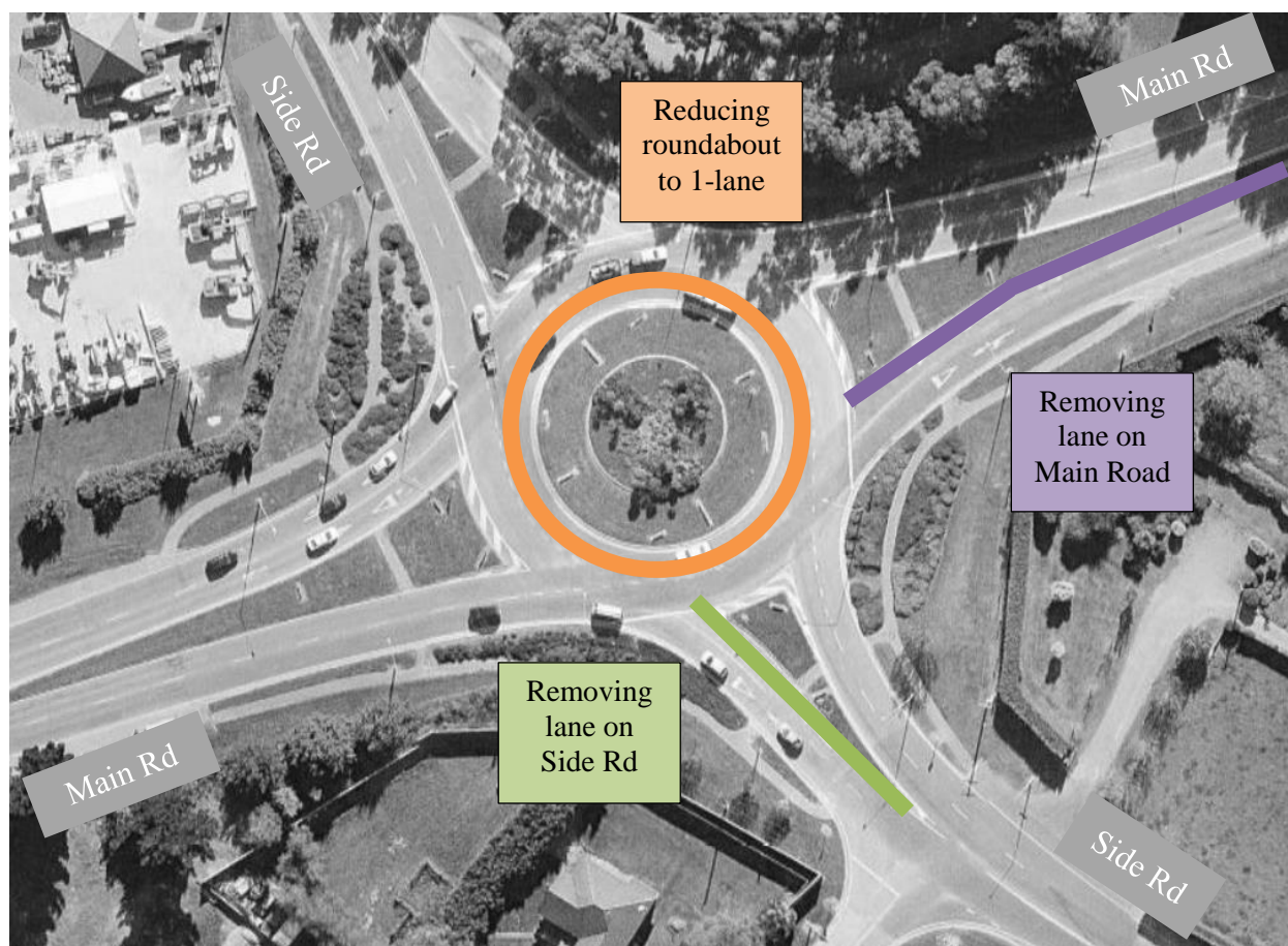
Figure 13: Example of Moderate 2-lane Roundabout
