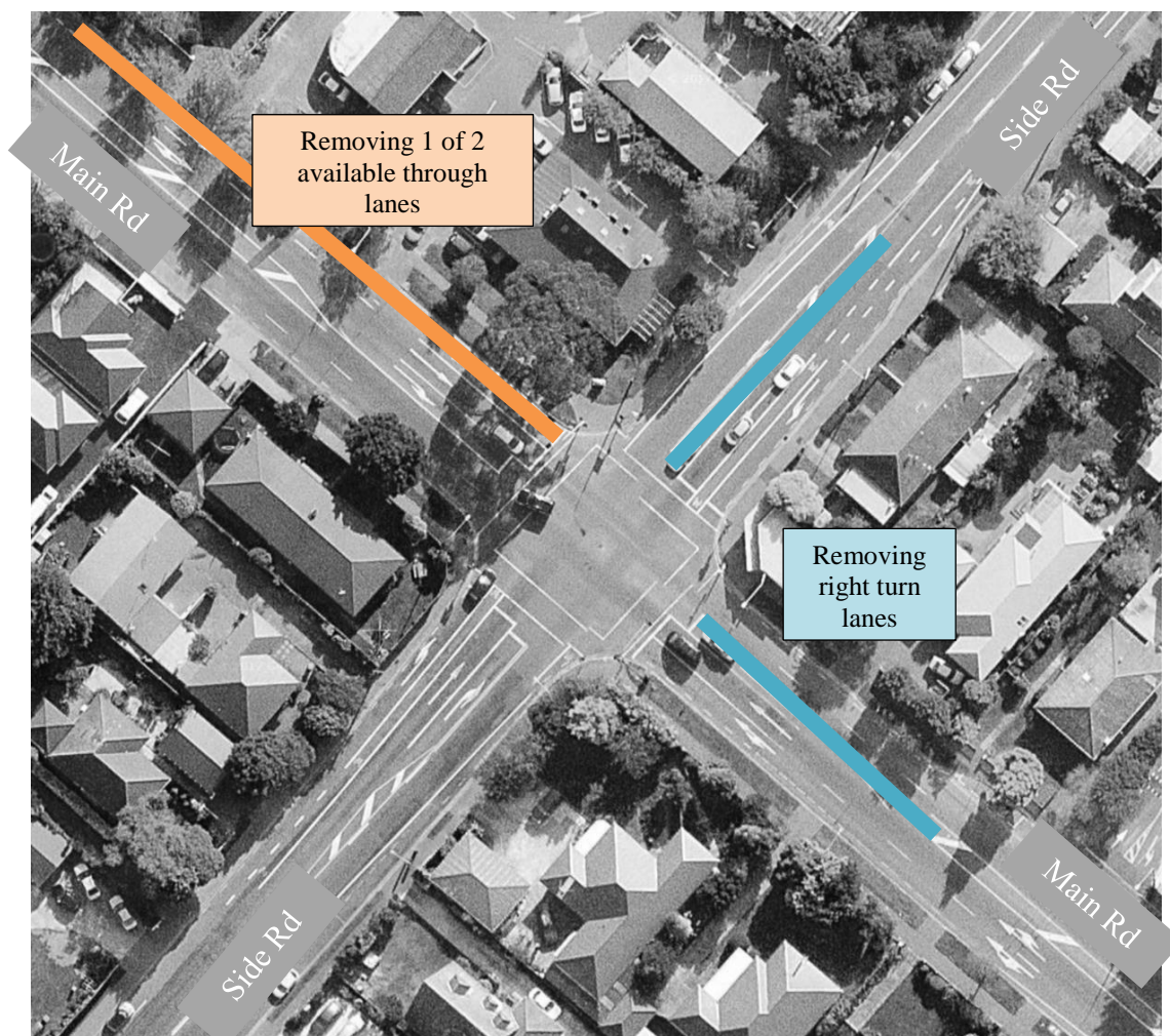
Figure 6: Typical 4-Way Moderate Signals
