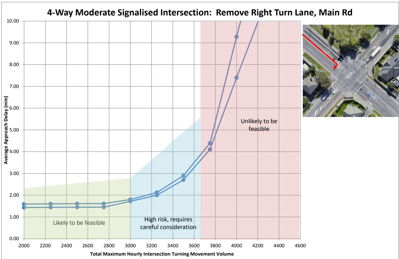
Figure 8: 4-way Moderate Signalised Intersection: Removing Right Turn Lane from Main Road
