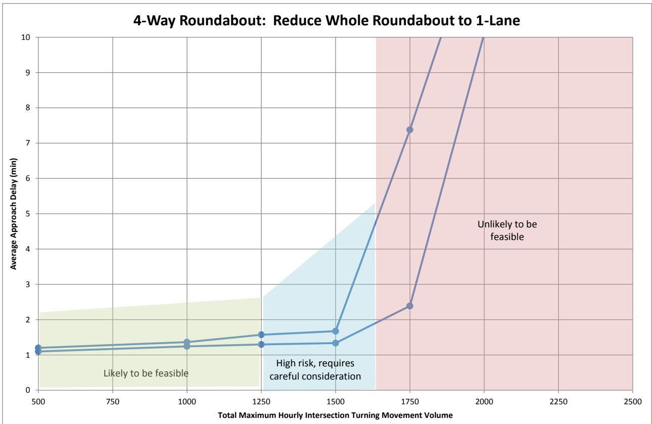
Figure 16: 2-lane 4Way Roundabout: Reducing Whole Roundabout to 1-lane
