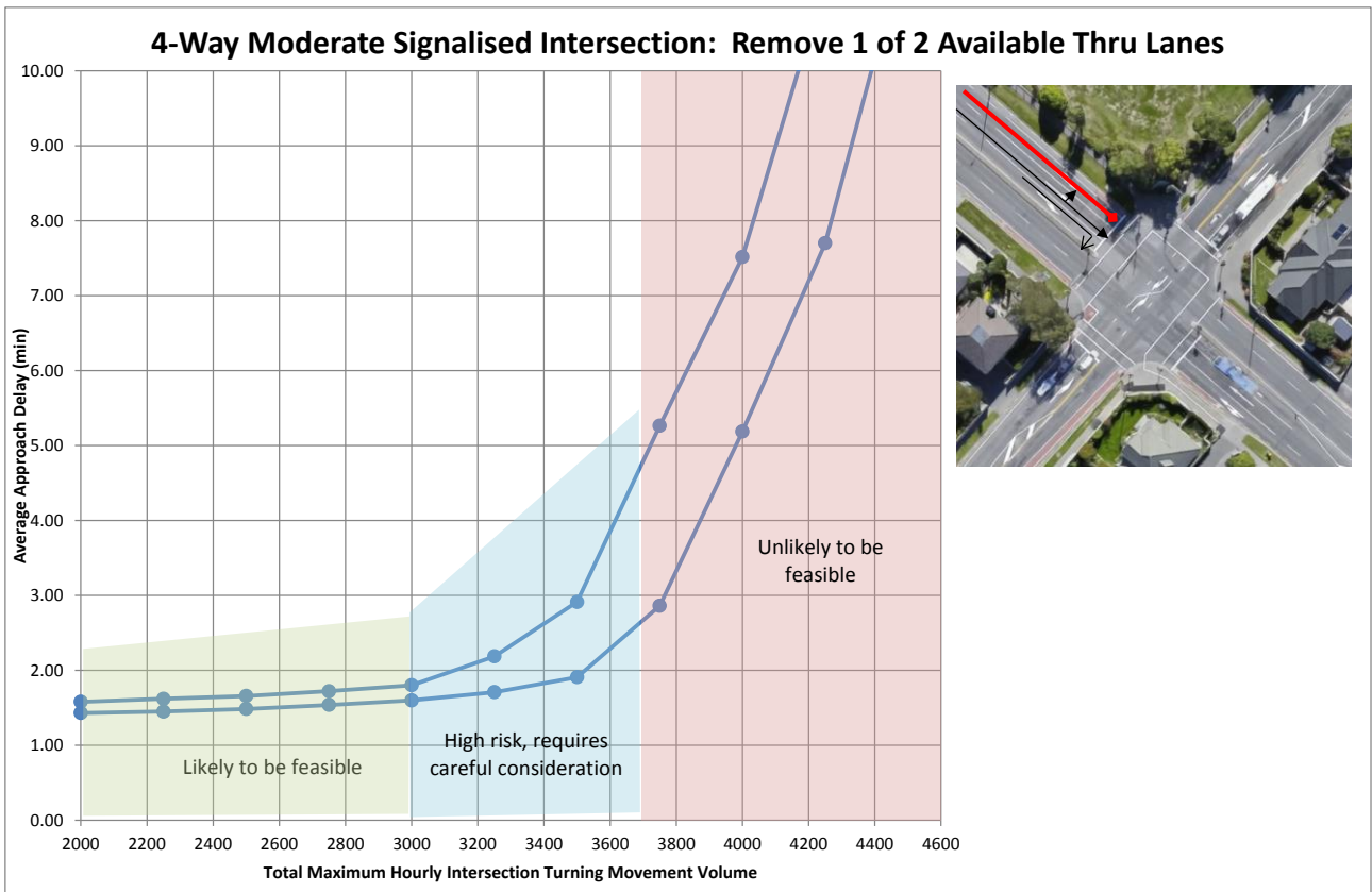
Figure 7: 4-Way Moderate Signalised Intersection: Removing 1 Through Lane
