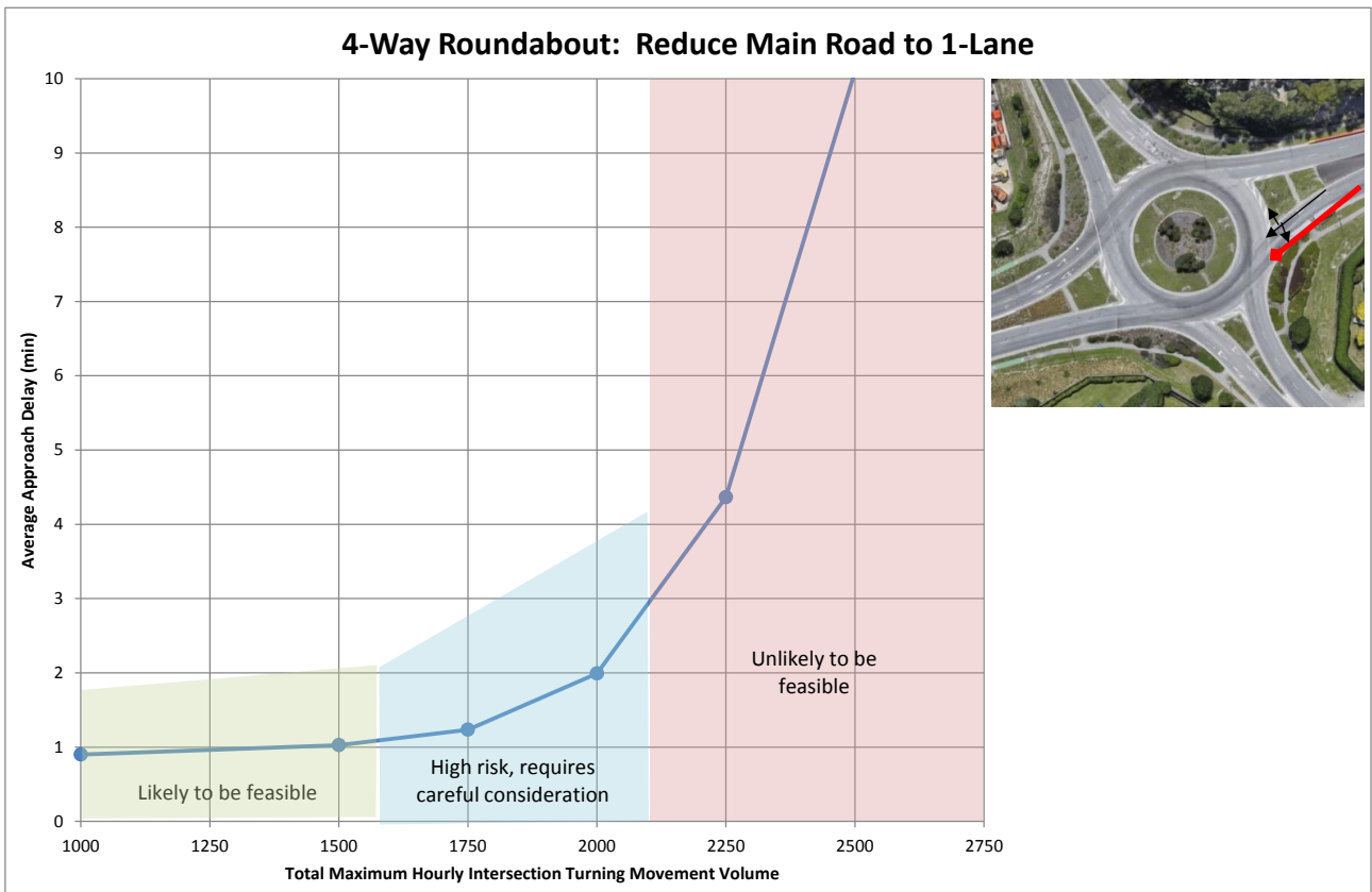
Figure 15: 2-lane 4Way Roundabout: Reducing Main Road to 1-lane
