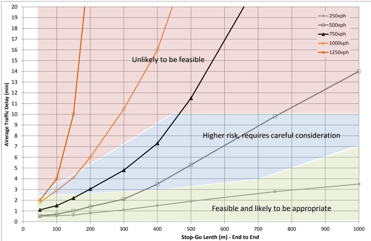
Figure 2: Capacity of Two-Way Traffic Flow through One-Lane Section
