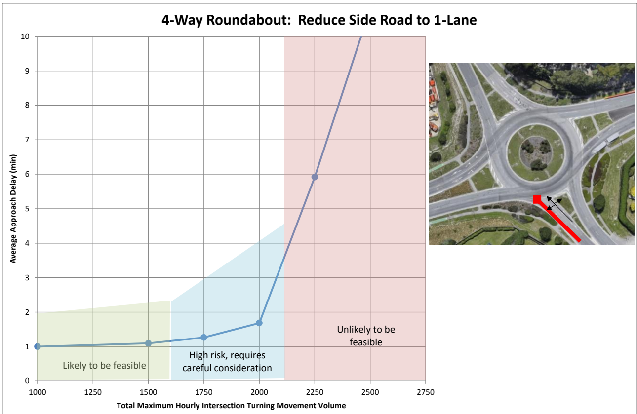
Figure 14: 2-lane 4Way Roundabout: Reducing Side Road to 1-lane
