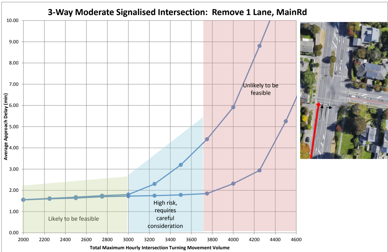
Figure 12: 3-Way Moderate Signals: Remove 1 Lane on Main Road
